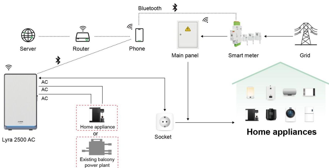
Figure 1-2 Network diagram
