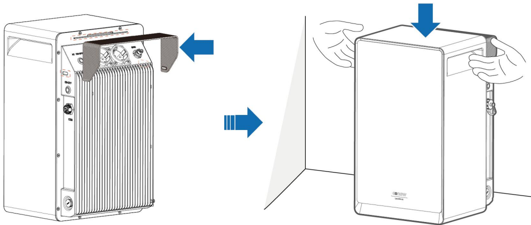
Figure 3-1 Installing the Lyra 2500 AC
