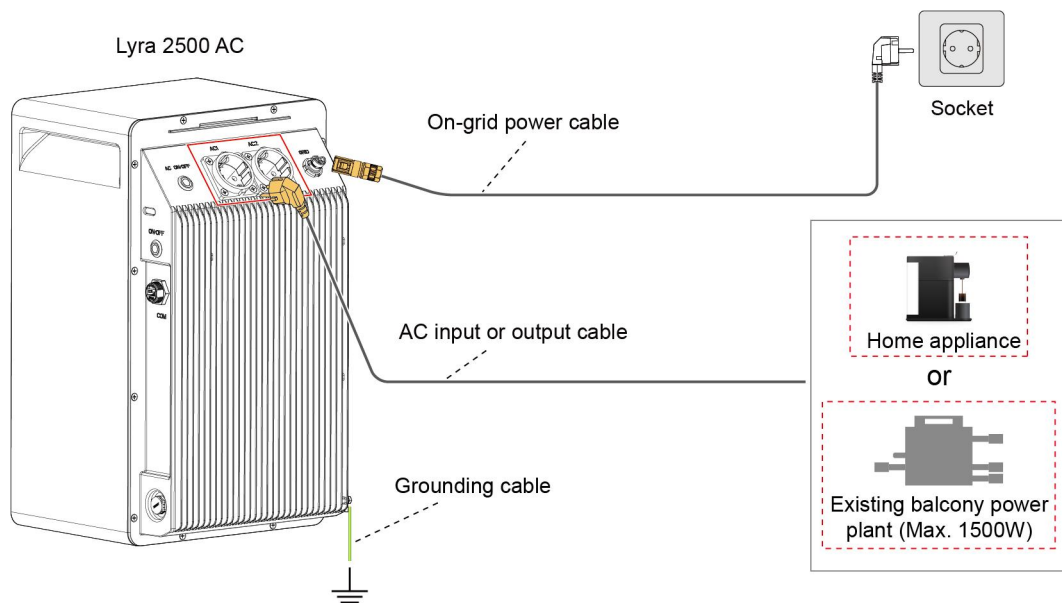
Figure 4-1 Installing the cables
