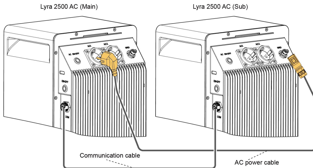
Figure 6 Installing the parallel cables
