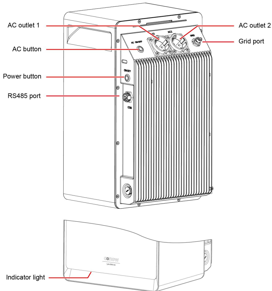
Figure 2-2 Lyra 2500 AC
