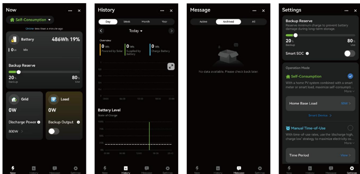
Figure 5-2 Device page
