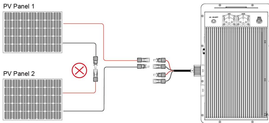
Figure 4-2 Do not connect in series
