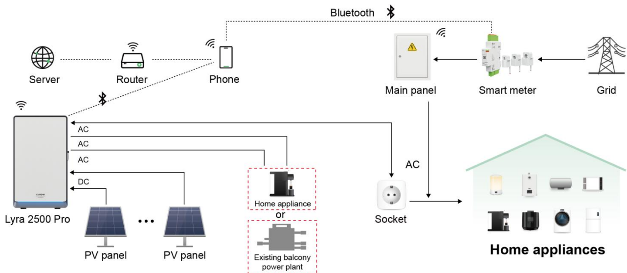
Figure 1-2 Network diagram
