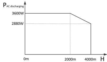
AC discharging power Vs altitude
